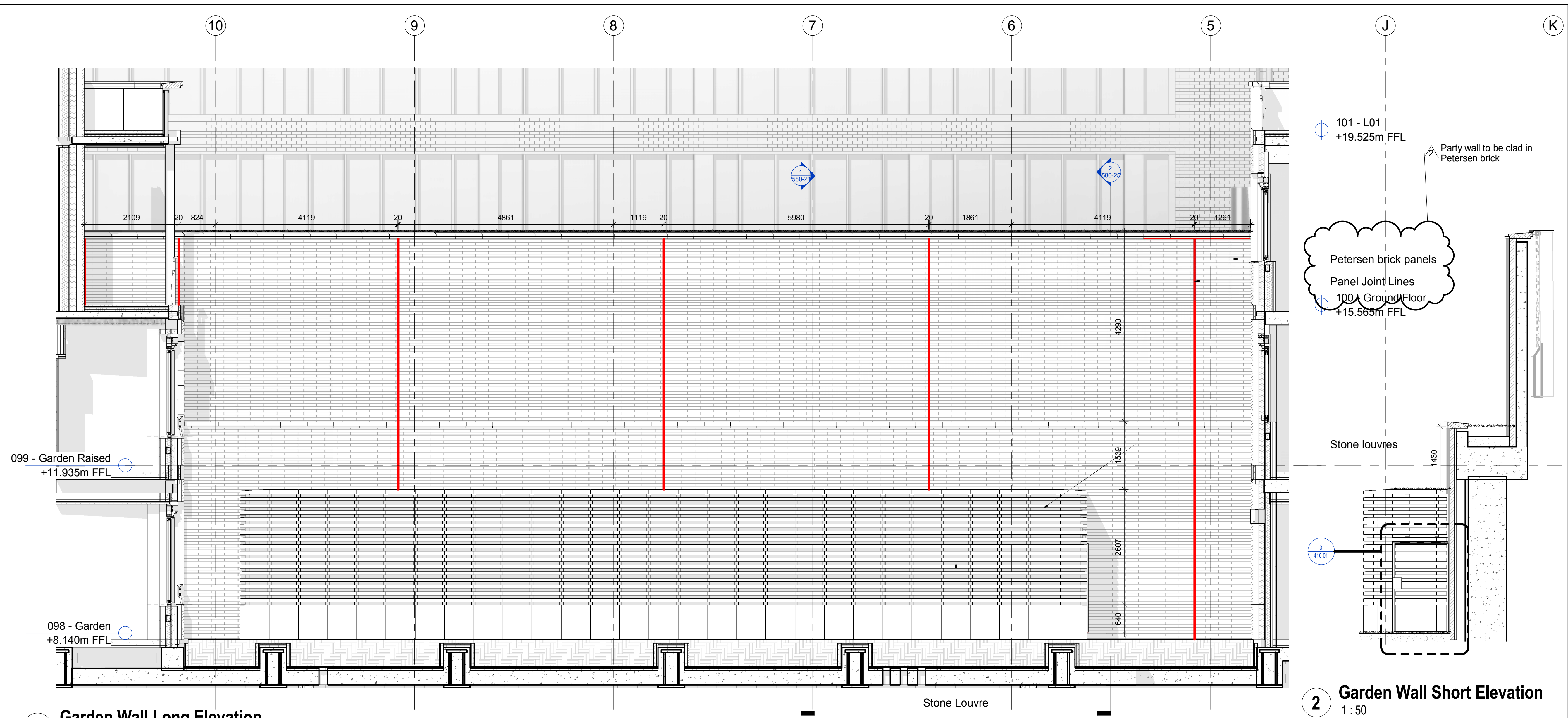
1 Garden Wall Long Elevation 1 : 50
